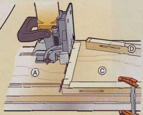
DRAWING 3 Cutting biscuit slots in the sides for receiving the fixed shelf
